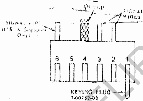
HEADER CONFIGURATION FOR OLDER COMPUTER ASSEMBLY 6-50458-XX at P103
