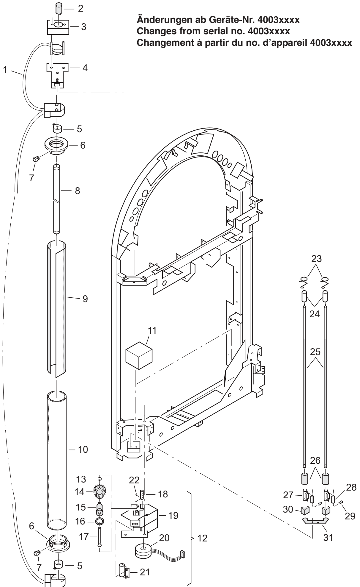
Fig. 4.2 - Tür - Beleuchtung / Door illumination / Porte - illumination
