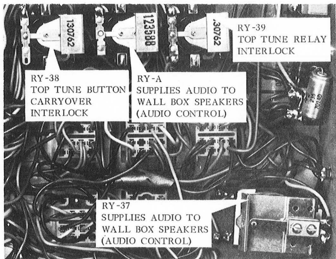
268 STEPPER Figure 2.
