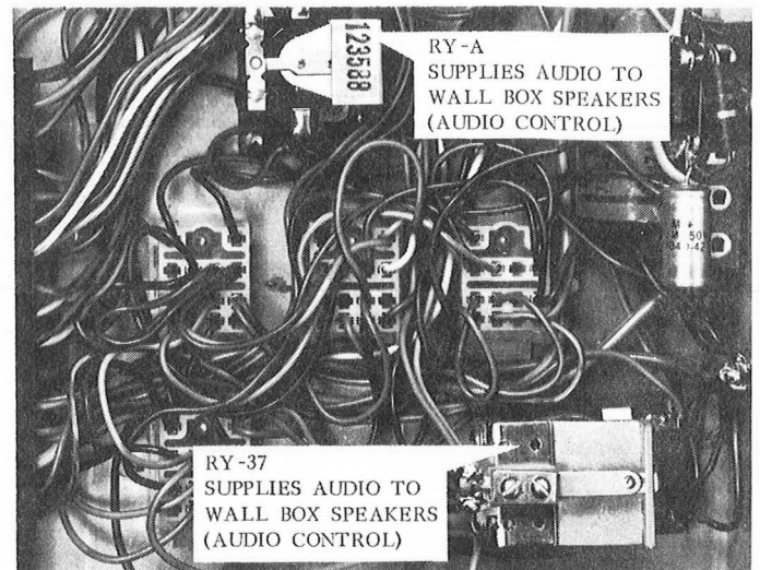
269 STEPPER Figure 3.
