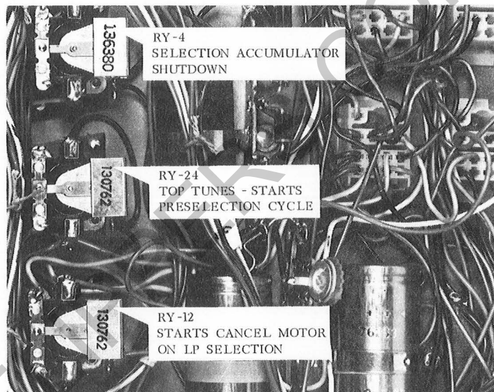
JUNCTION BOX Figure 1.
