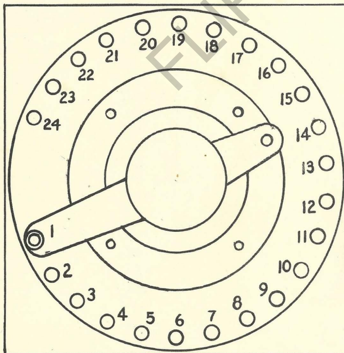
Figure 1 - Contact Disc
